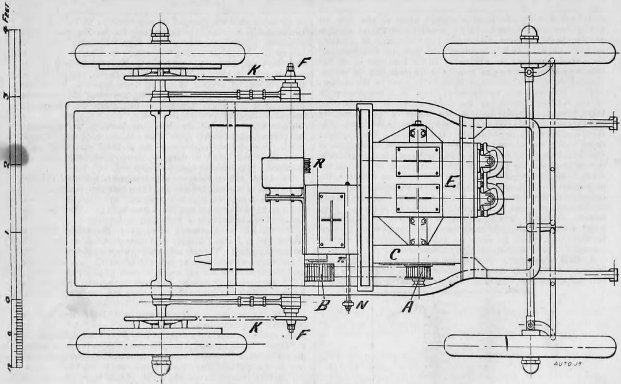
FIGS. 2 and 3.—The 10-h.p. Wolseley Car—Elevation and Plan.
